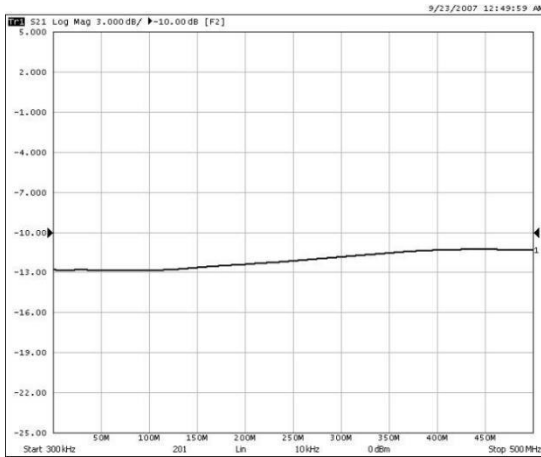
DC-500M Frequency Response Curve Test Diagram
